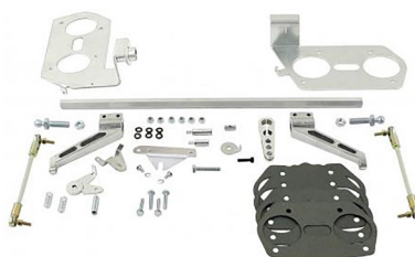
Cross-bar linkage Weber IDF, Dellorto DRLA Type-1 engines, Type-3 engines
