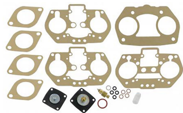
Carburetor rebuild/gasket kit Weber IDF 40, IDF 44, EMPI HPMX 40, HPMX 44
