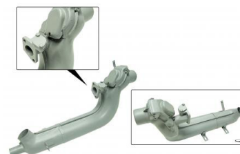
Heat exchanger right Type-3 engines
