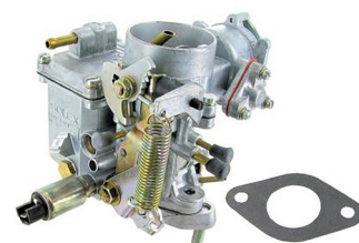
H30/31 PICT carburetor A-quality Type-1 engines and replaces the Solex 30 PICT-1, 30 PICT- 2, 30 PICT-3, 31 PICT-3, 31 PICT-4
