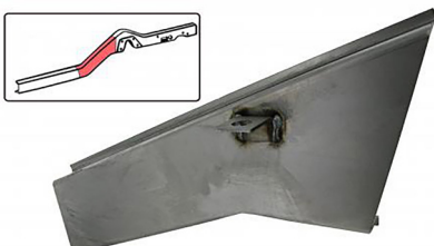
Front side member repair section right Bus until 7.1967
