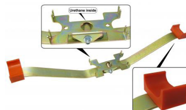
Sway bar rear (camber stop) Beetle with swing axle 8.1960 and later, Karmann Ghia with swing axle 8.1960 and later, Bus 6.1959 until 7.1967, Thing with swing axle
