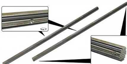
Axle beam torsion leaves (2 bundles of 9 leaves) Bus 4.1955 until 7.1979
