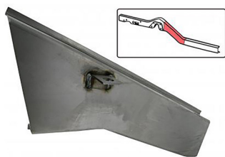
Front side member repair section left Bus until 7.1967
