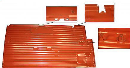
Cargo floor pan right Bus until 7.1967
