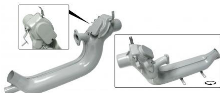
Heat exchanger standard right Type-1 engine 1.1963 and later (except 30hp and AJ injection)
