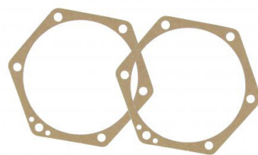
Swing axle adjusting gaskets 0.20 mm (per pair) Swing axle, Beetle/Karmann Ghia, Bus, Type 3, Thing
