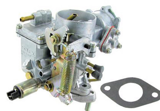
H30/31 PICT carburetor A-quality Type-1 engines and replaces the Solex 30 PICT-1, 30 PICT- 2, 30 PICT-3, 31 PICT-3, 31 PICT-4
