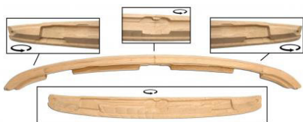
Wooden hood frame front beam Karmann Ghia convertible until 1968 (VIN 149 431 007)
