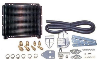
Oil cooler kit 72 plates 280 x 260 x 40mm
