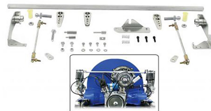
Carburetor cross-bar linkage Weber ICT Type-1 engines
