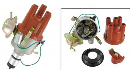
Distributor with vacuum advance Type-1 engines with Solex carburetor 30 PICT-3, 31 PICT-3, 31 PICT-4, 34 PICT-3, 34 PICT-4
