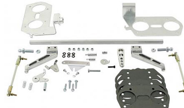
Cross-bar linkage Weber IDF, Dellorto DRLA Type-1 engines, Type-3 engines
