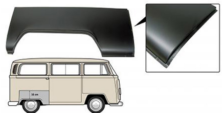
Rear wheel arch repair panel right Bus 8.1970 until 7.1979
