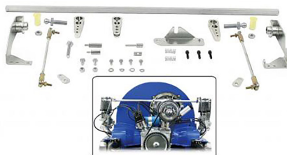
Carburetor cross-bar linkage Weber ICT Type-1 engines
