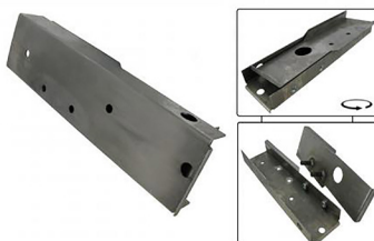
Rear side member (repair section) left Bus 8.1971 until 7.1979
