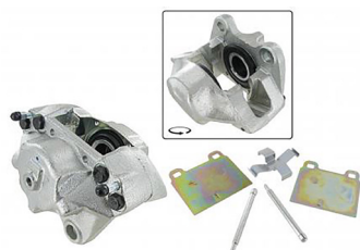
Brake caliper left Bus 8.1972 until 7.1979
