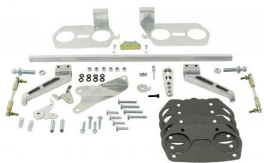
Cross-bar linkage Weber IDF, Dellorto DRLA Type-4 engines
