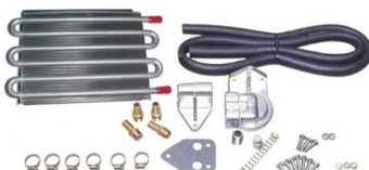
6 pass oil cooler kit 300 x 190 x 60mm
