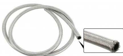
Oil hose with braided stainless steel outer jacket (per meter) Inner diameter: 12.7mm, Outer diameter: 17mm
