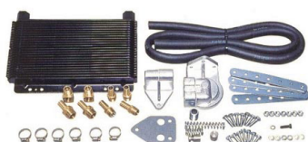
Oil cooler kit 48 plates 280 x 190 x 40mm
