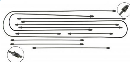
Brake line kit (10-part) Bus 8.1972 until 1972 (VIN 293 2044 831) LHD
