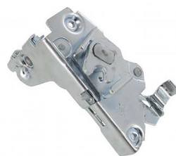
Cabin door lock mechanism right Bus 8.1973 until 7.1979
