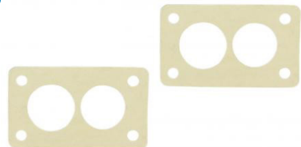
Carburetor base gasket (per pair) Weber 32/36 DFEV, DFEV, EMPI EPC 32/36F, Holley 5200
